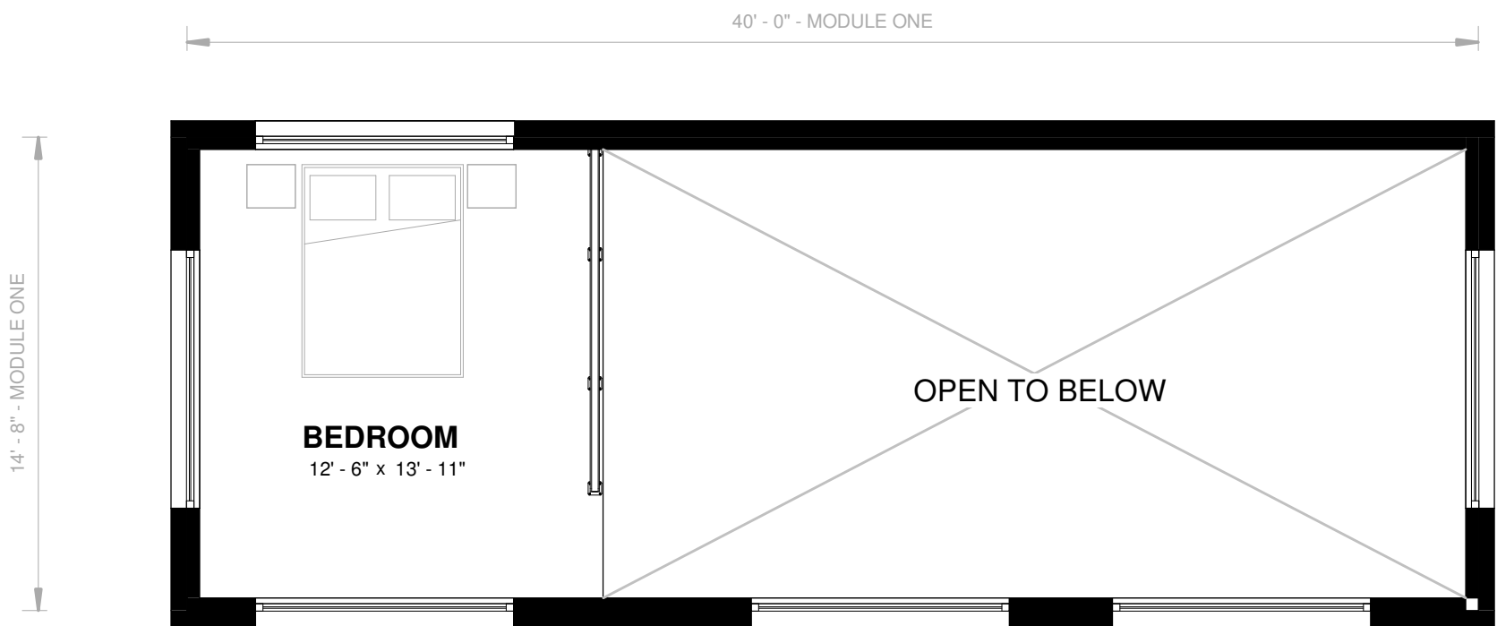
LOFT FLOOR
